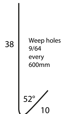
Starter Strip
