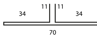
T Section
