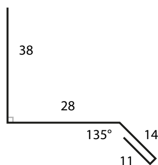
Drip Mould
