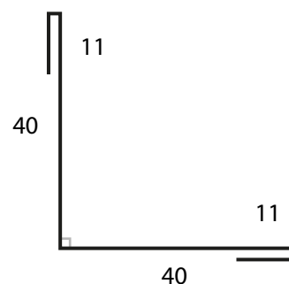
40mm Internal 90°
